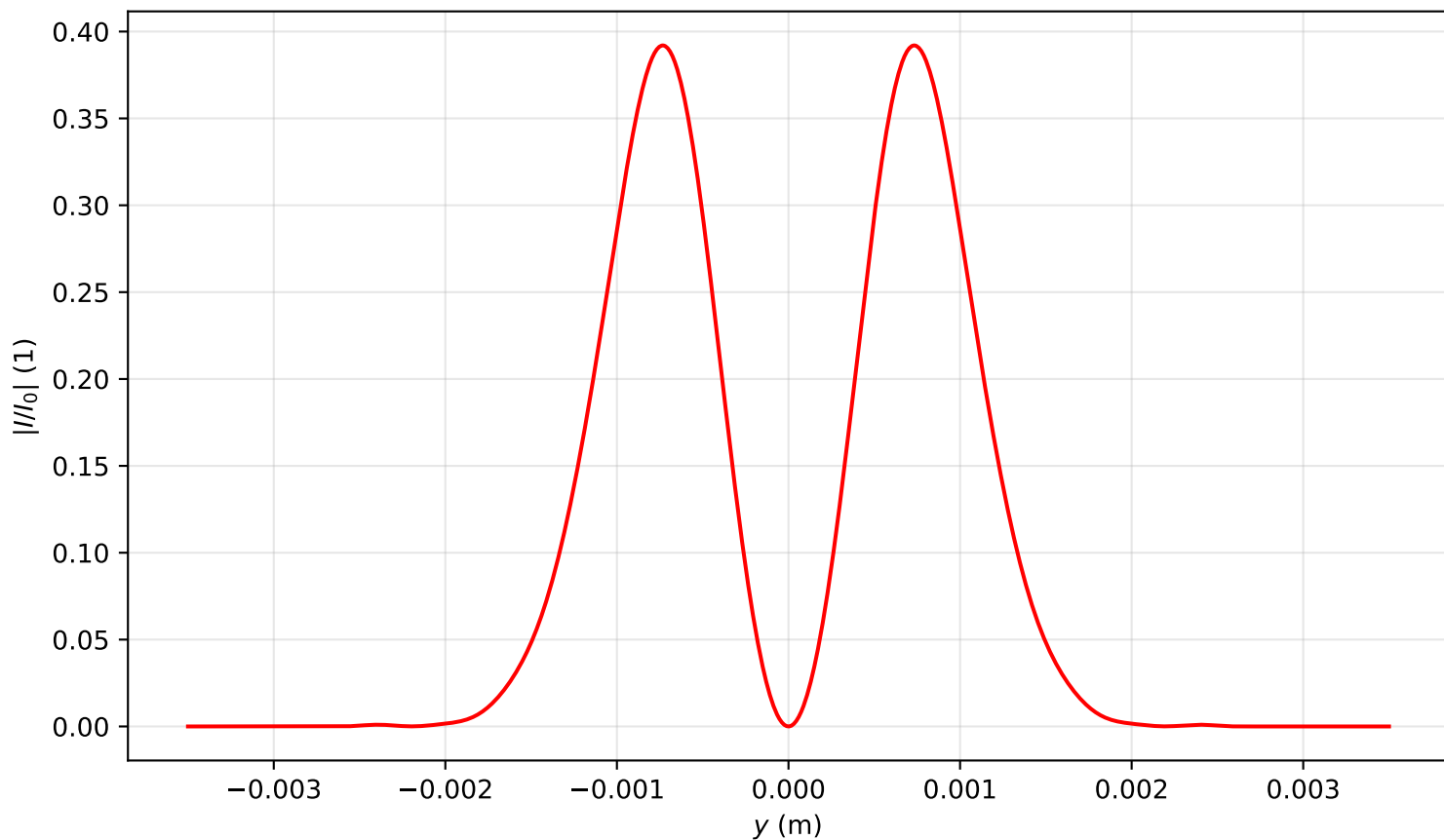
Intensity profile I(x=0, y, z=2.468)/I_0 , P_{in}=2.0P_{cr} , artificial time
